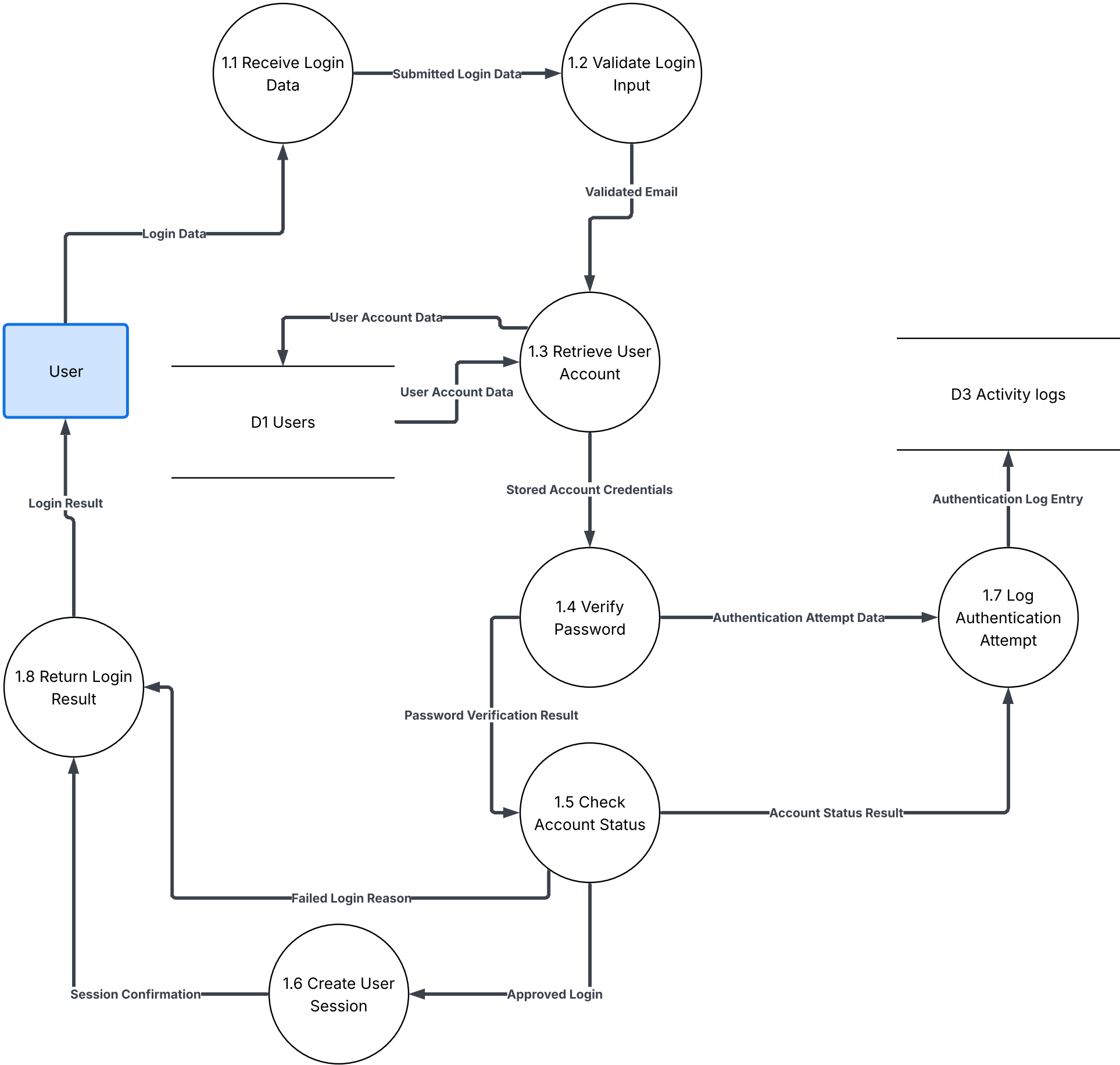
Data Flow Diagram Level 2: Process 1.0 Authenticate User
